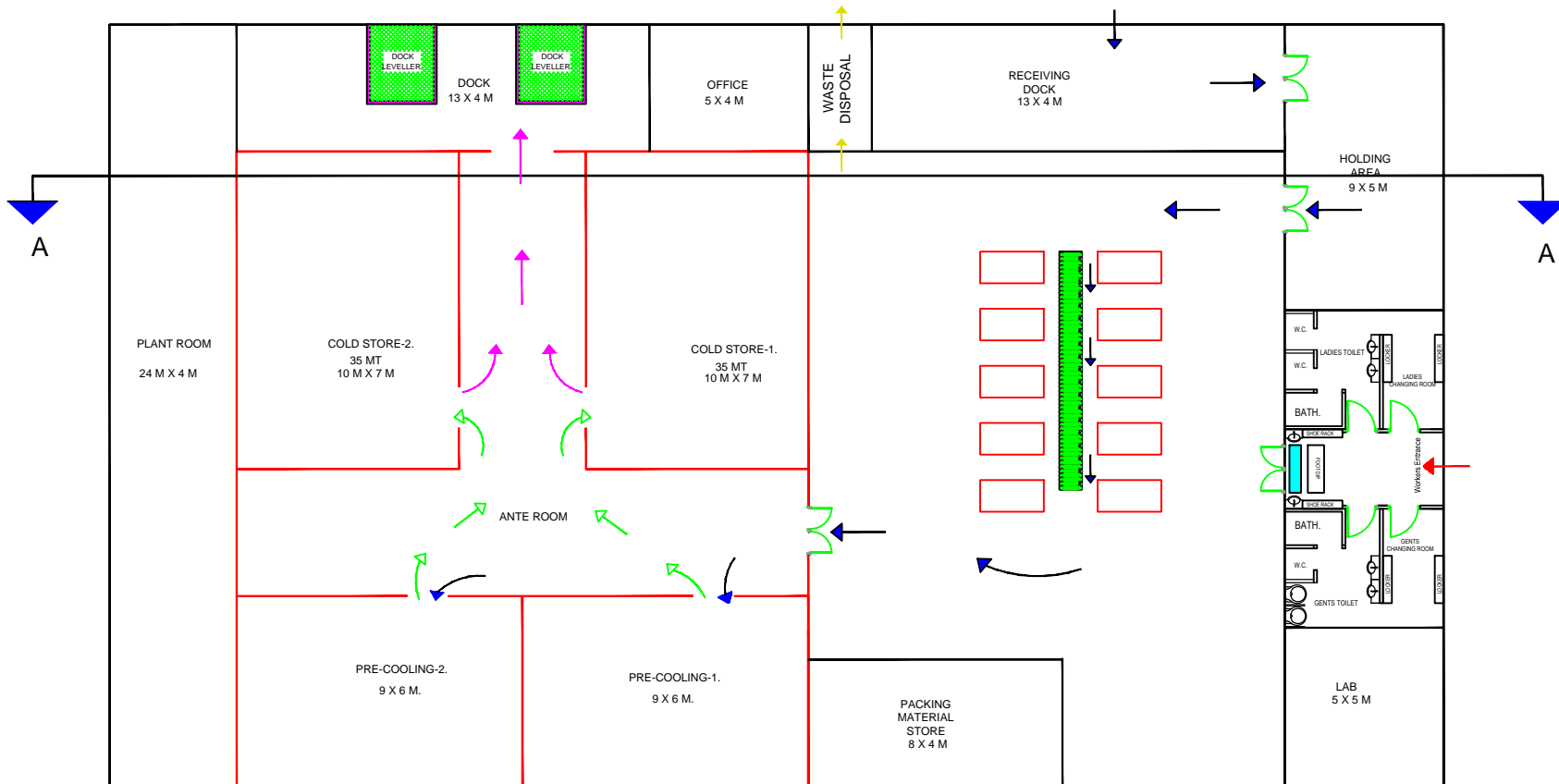
EXPORT ORIENTED PACKHOUSE FOR SAPOTA (2MT/HR CONVEYOR LINE WITH GRADING/SORTING TABLES) LARGE FACILITY
