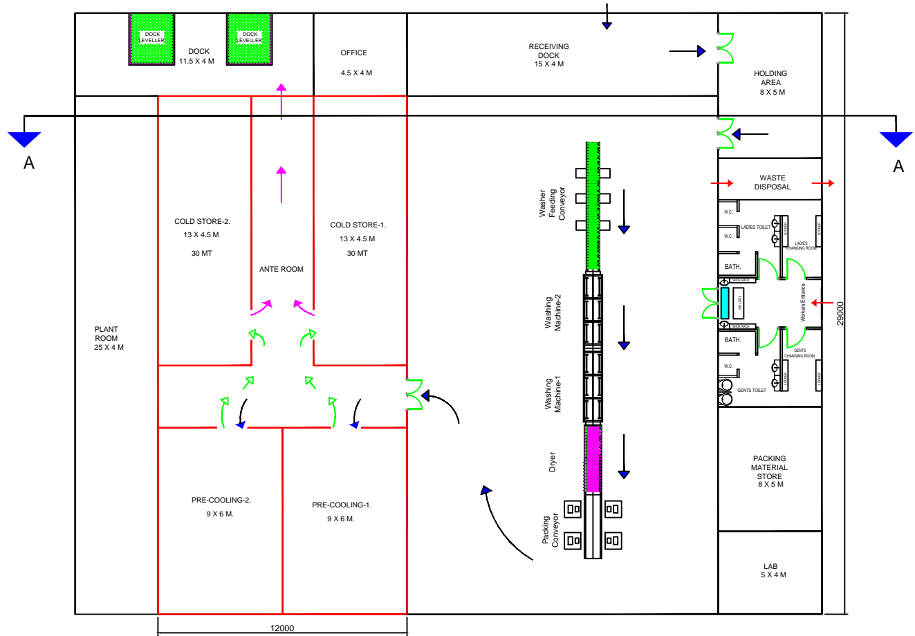
EXPORT ORIENTED PACKHOUSE FOR BANANA (2MT/HR WASHING/DISINFECTING/DRYING LINE) LARGE FACILITY
