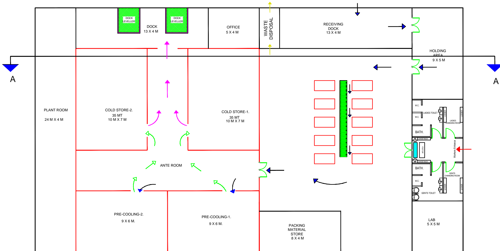
EXPORT ORIENTED PACKHOUSE FOR CUSTARD APPLE (2MT/HR CONVEYOR LINE WITH GRADING/SORTING TABLES) LARGE FACILITY
